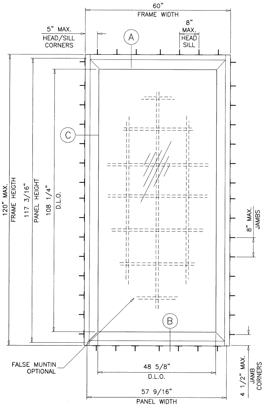
TYPICAL ELEVATION
