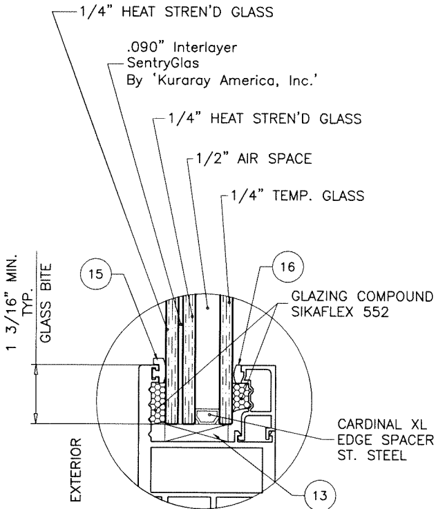
GLASS TYPE 'Ai' 1-3/8" OVERALL LAM. INSUL. GLASS
