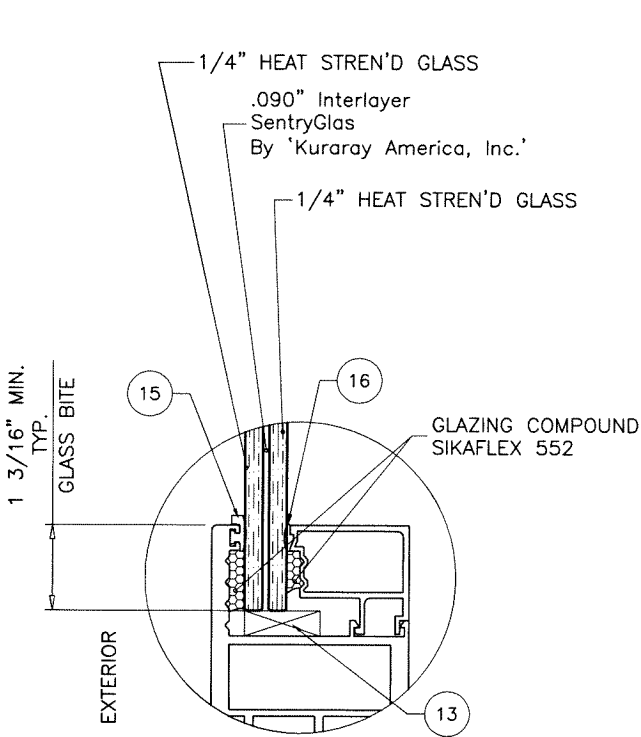
GLASS TYPE 'A' 9/16" OVERALL LAMINATED GLASS
